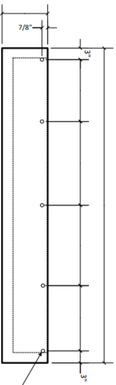
Section End View
